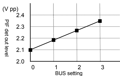
Graph PIF det out level
