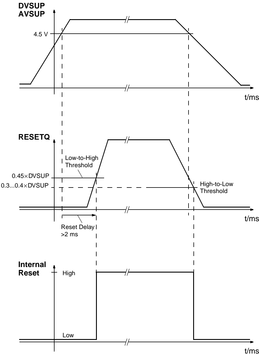
Fig. 4–26: Power-up sequence
