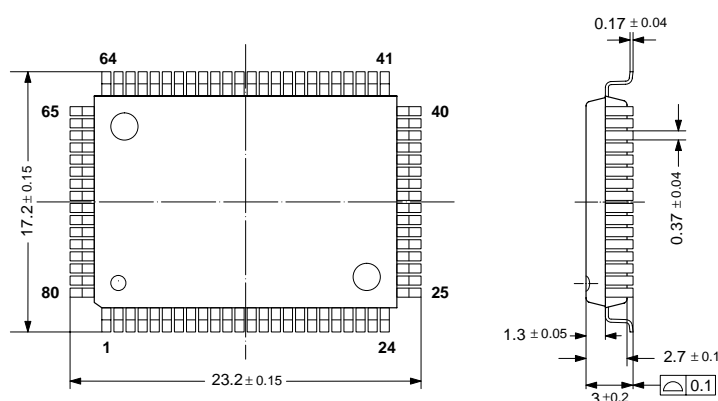
Fig. 4-3: 80-Pin Plastic Quad Flat Pack Package (PQFP80)
