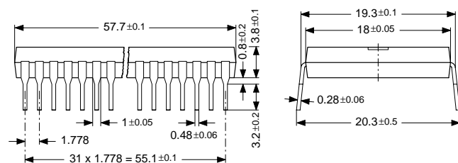
Fig. 4-1: 64-Pin Plastic Shrink Dual Inline Package (PSDIP64)
