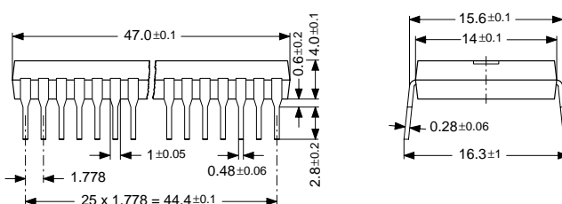
Fig. 4-2: 52-Pin Plastic Shrink Dual Inline Package (PSDIP52)
