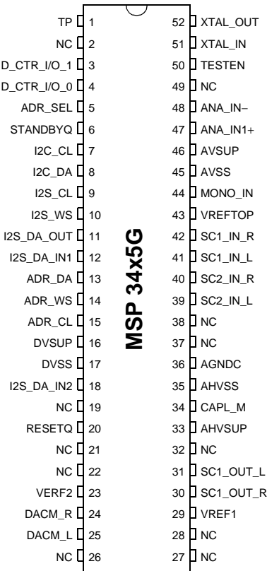
Fig. 4–7: PSDIP52 package
