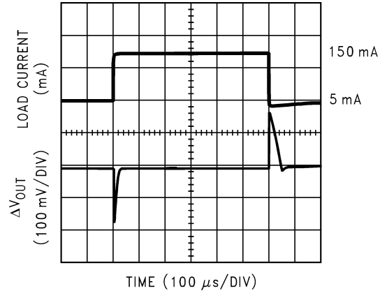
Load Transient Response @ V_{IN} = 4.2V , C_{OUT} = 1\mu F
