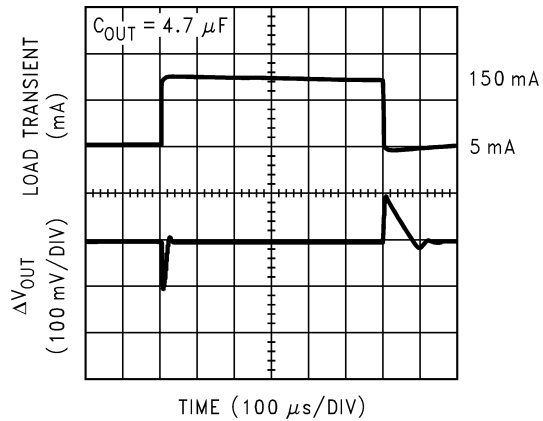
Load Transient Response @ V_{IN} = 3.1\text{V}
