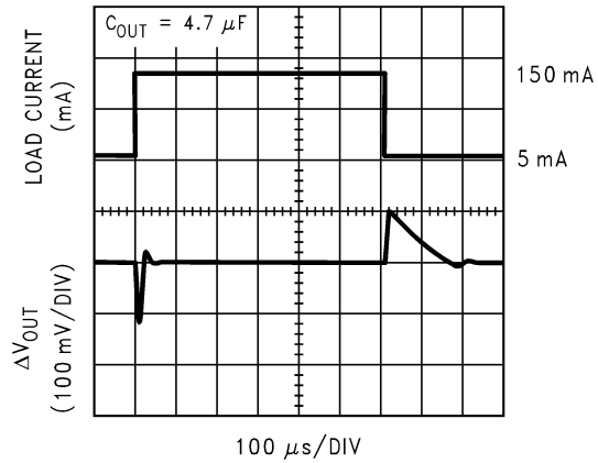
Load Transient Response @ V_{IN} = 3.6\text{V}
