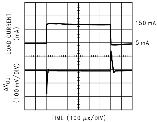
Load Transient Response @ V_{IN} = 3.1\text{V} , C_{OUT} = 1\mu\text{F}
