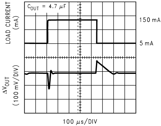
Load Transient Response @ V_{IN} = 3.35\text{V}
