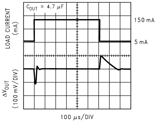
Load Transient Response @ V_{IN} = 4.2\text{V}
