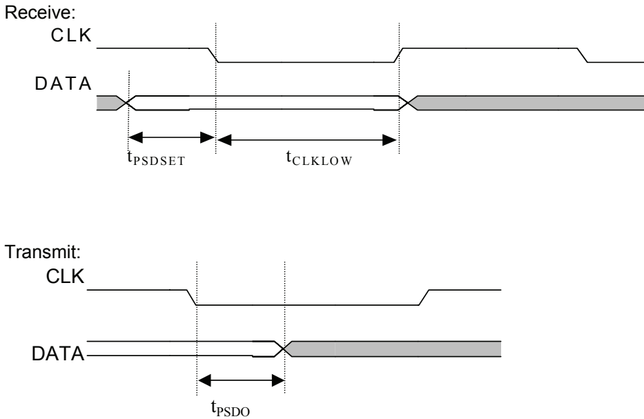
Figure 10-14. PS/2 Receive/Transmit Timing
