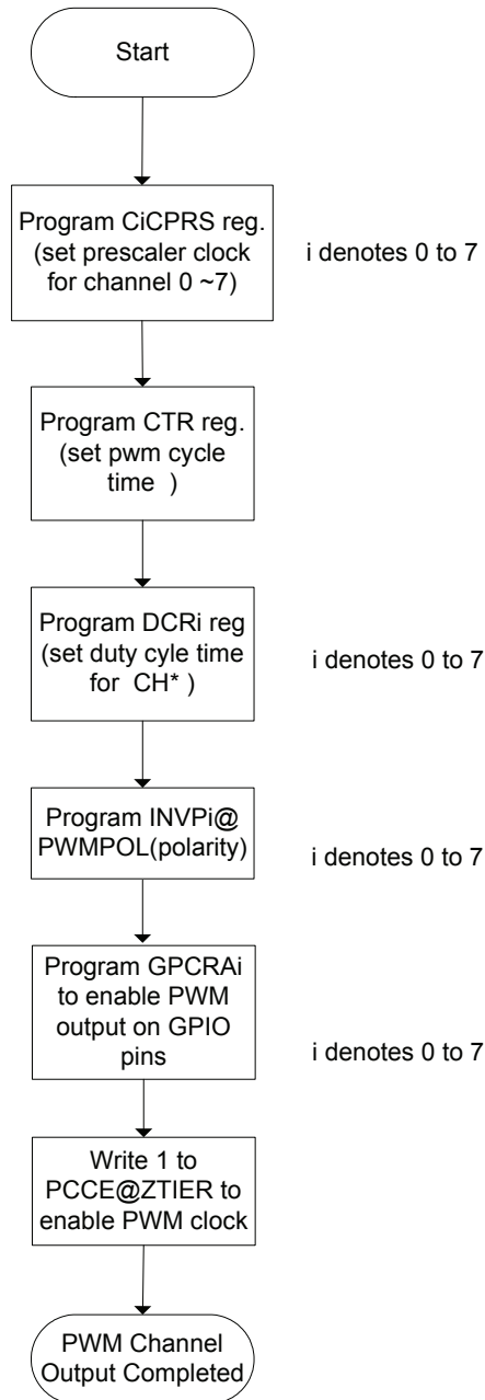
Figure 7-28. Program Flow Chart for PWM Channel Output
