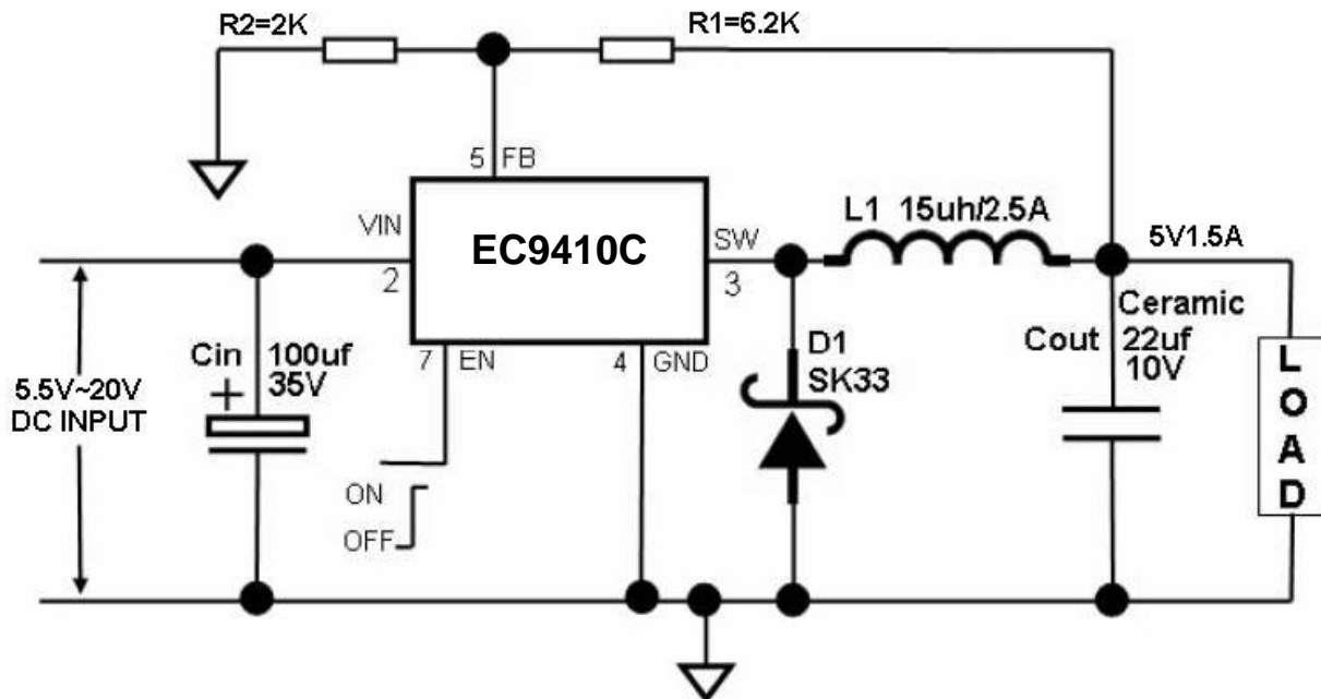
Typical Application Circuit (with ceramic output capacitor) @ 5V/1.5A
