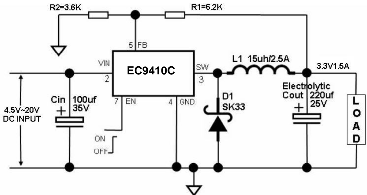
Typical Application Circuit @ 3.3V/1.5A
