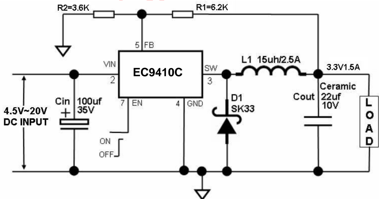
Typical Application Circuit (with ceramic output capacitor) @ 3.3V/1.5A
