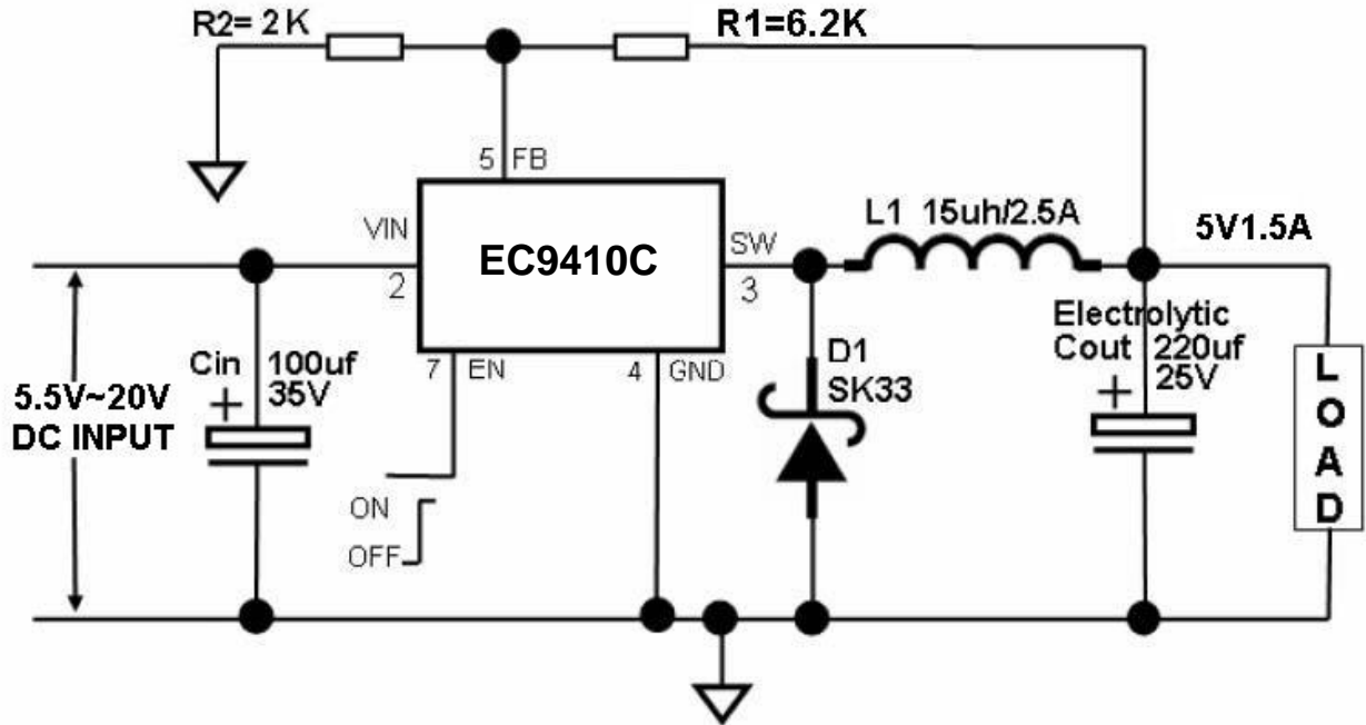
Typical Application Circuit @ 5V/1.5A
