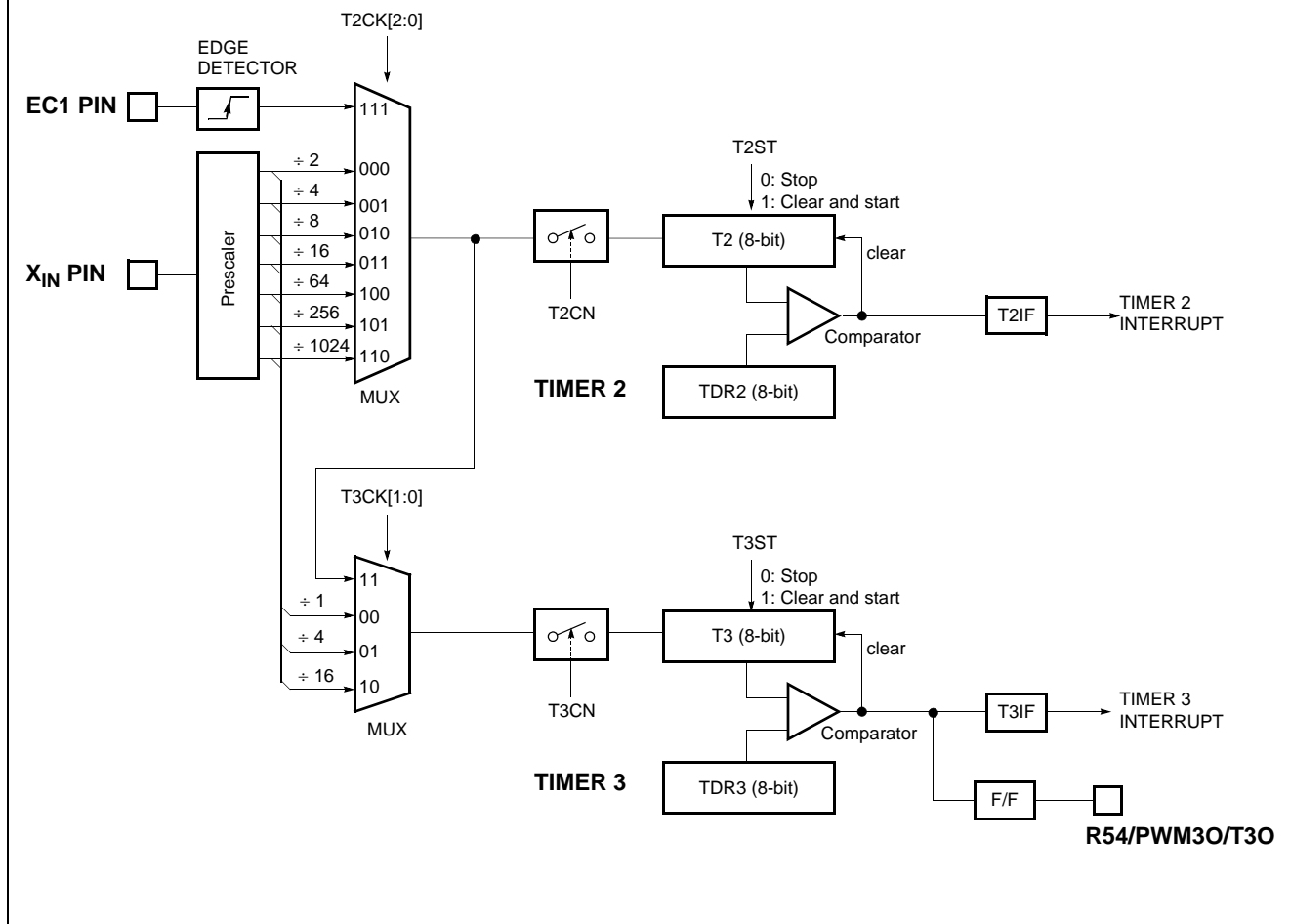
Figure 14-5 8-bit Timer/Counter 2, 3
