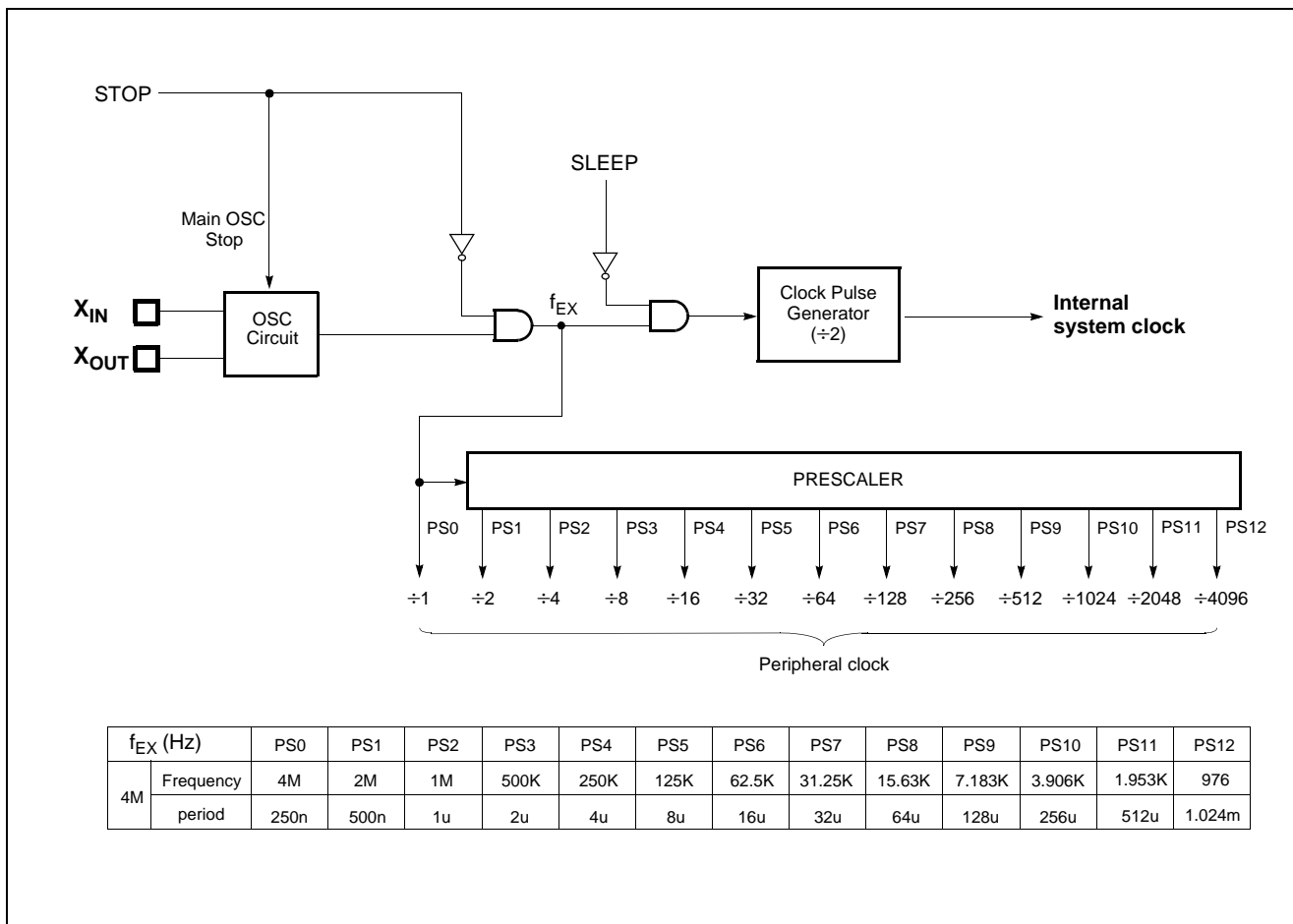
Figure 10-1 Block Diagram of Clock Generator
