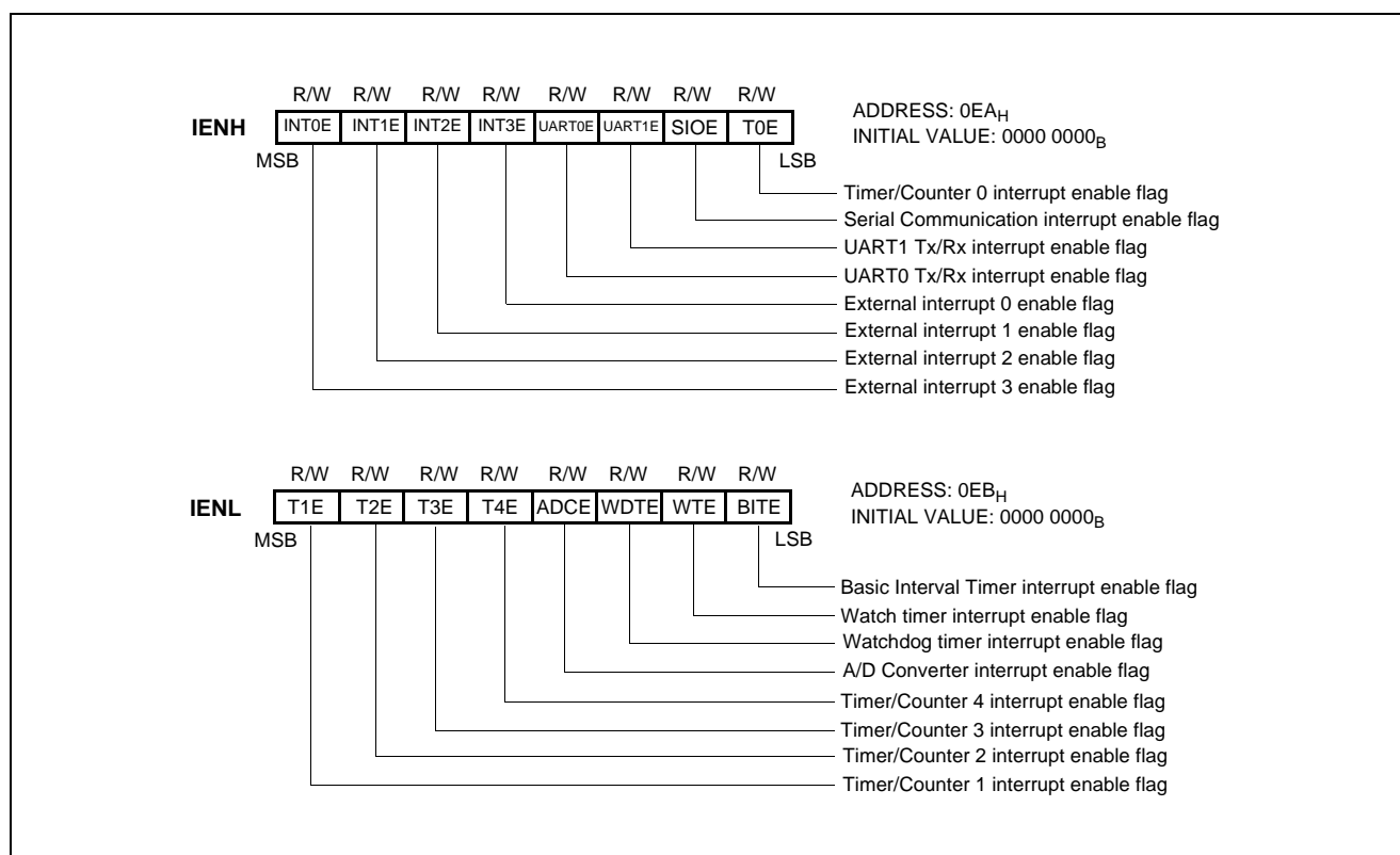
Figure 19-2 Interrupt Enable Flag Register
