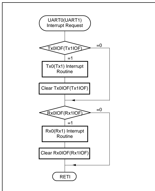
Figure 17-7 Shared Interrupt Vector of UART
