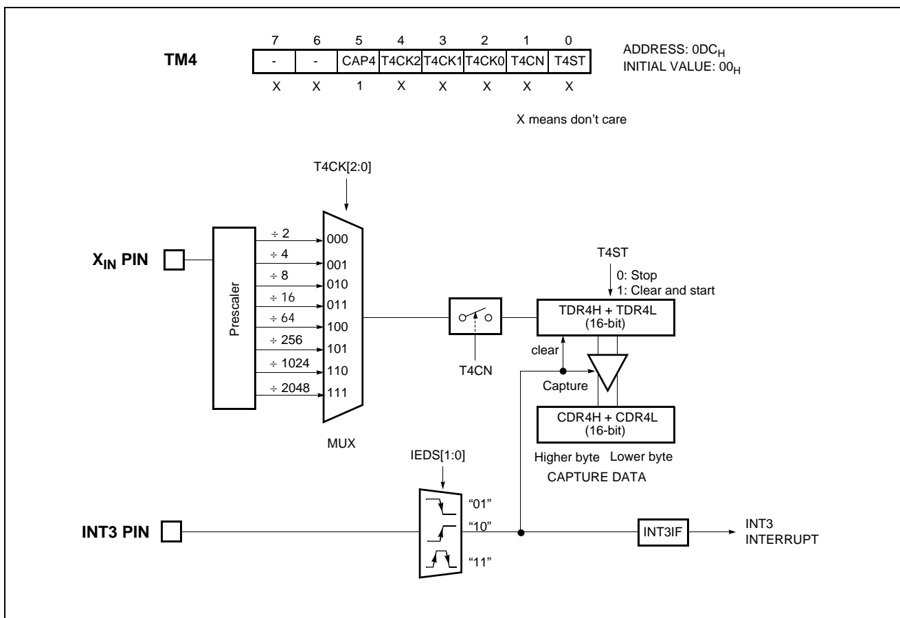
Figure 14-19 16-bit Capture Mode of Timer 4
