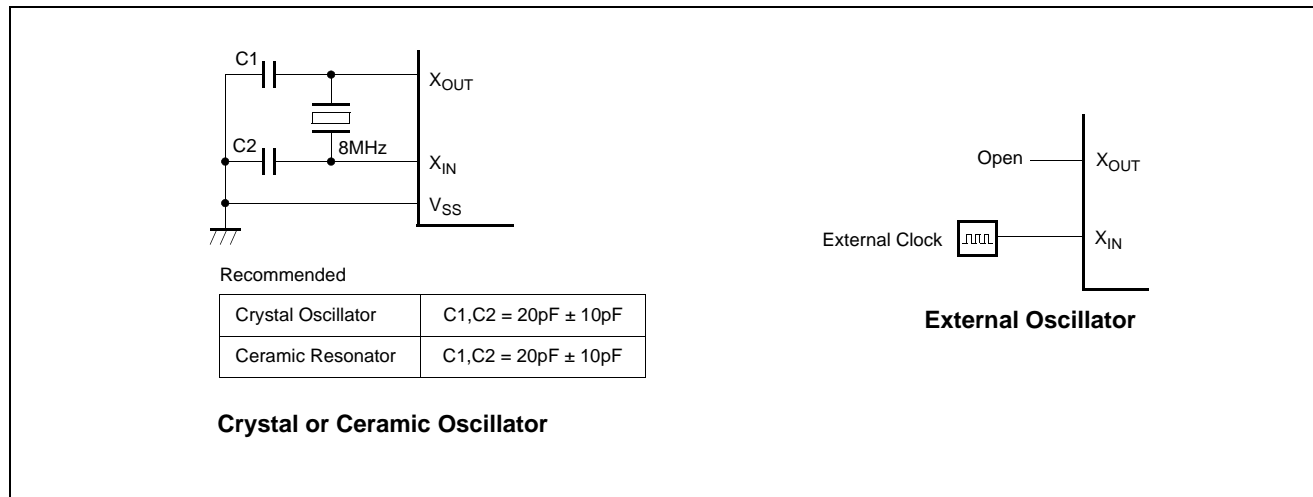
Figure 22-1 Oscillation Circuit
