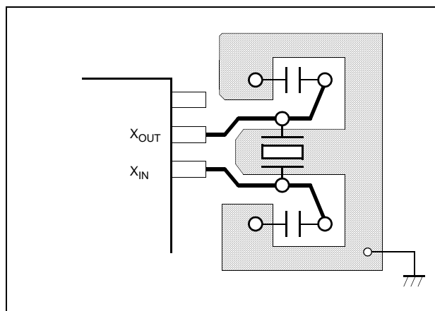
Figure 22-2 Layout of Oscillator PCB circuit
