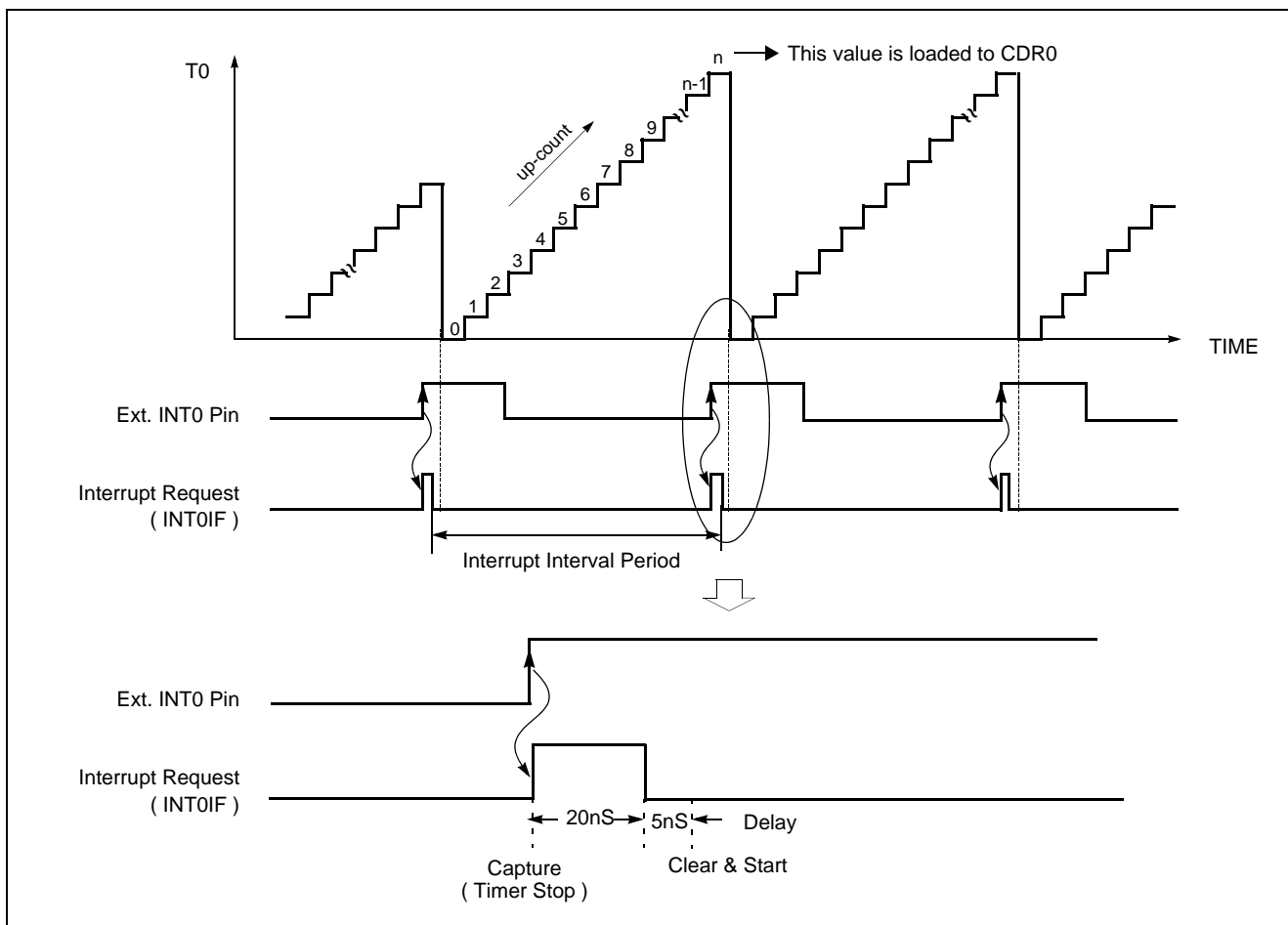
Figure 14-15 Input Capture Operation of Timer 0 Capture mode
