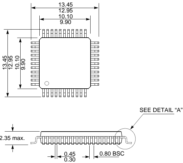
44MQFP
