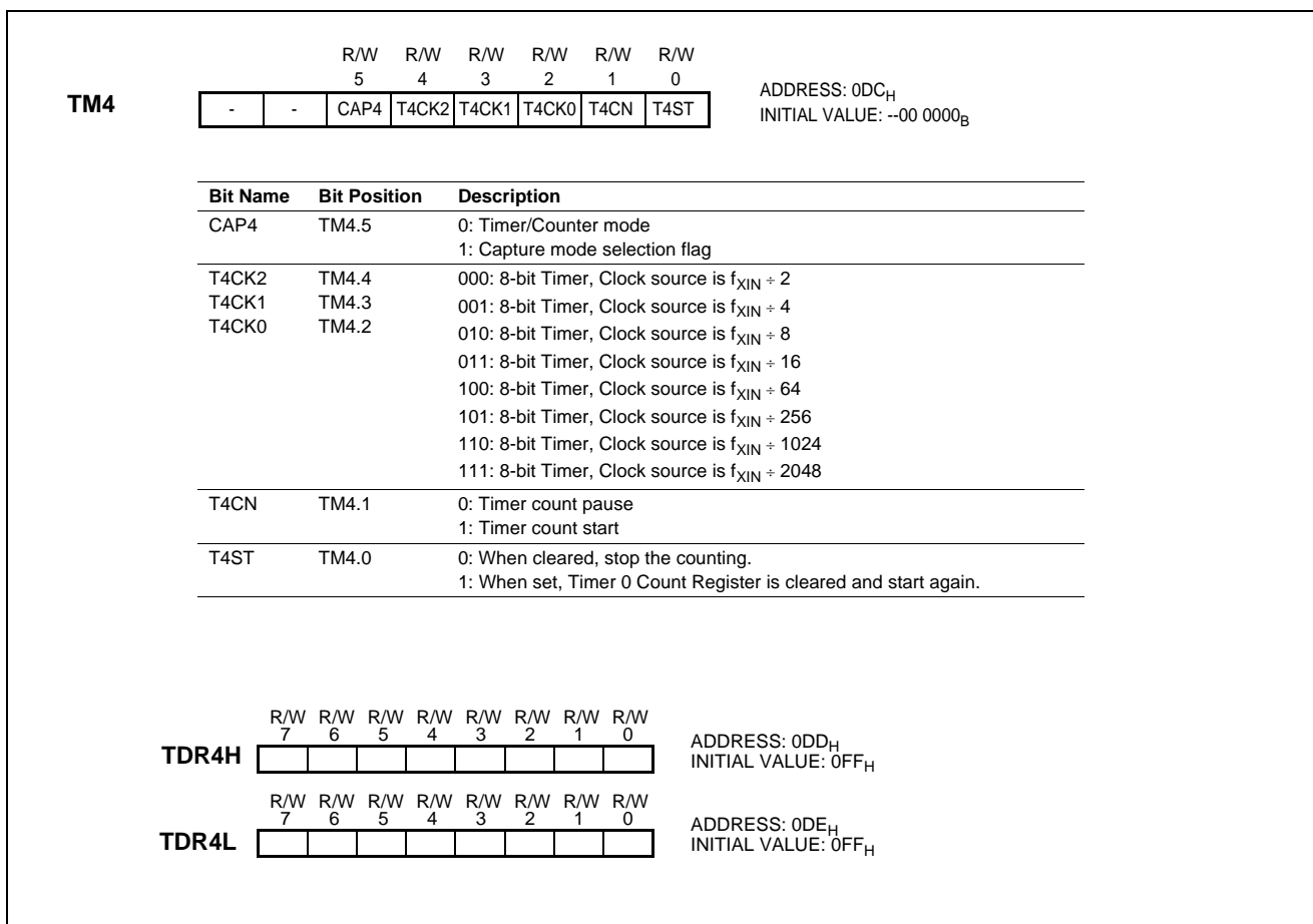
Figure 14-3 TM4 Register
