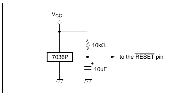
Figure 23-1 Simple Power-on-Reset Circuit
