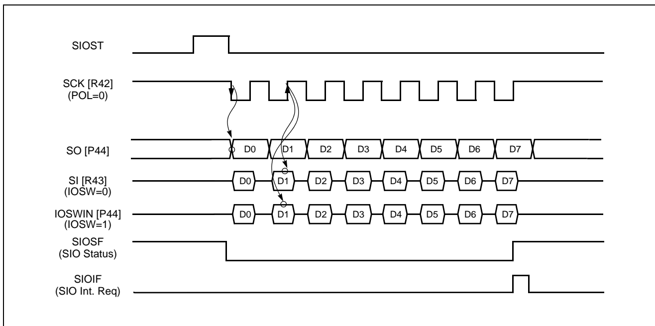
Figure 16-3 Serial I/O Timing Diagram at POL=0
