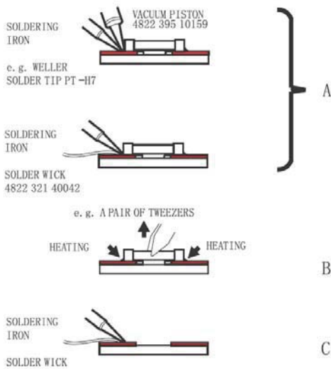
Fig. 1 DISMOUNTING
