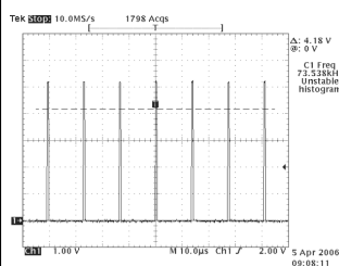
1 H-SYNC
