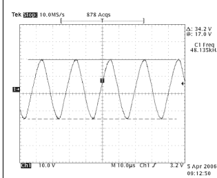
3 LAMP CURRENT
