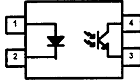
(2) 2561 (IC102)
