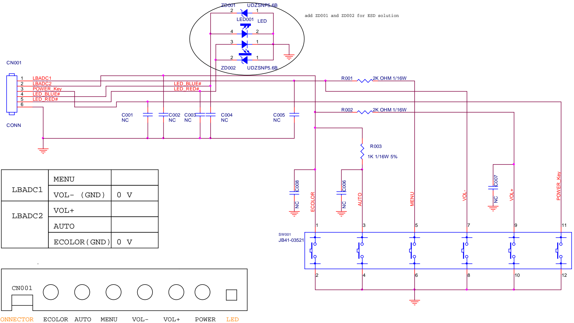
CONNECTOR ECOLOR AUTO MENU VOL- VOL+ POWER LED
